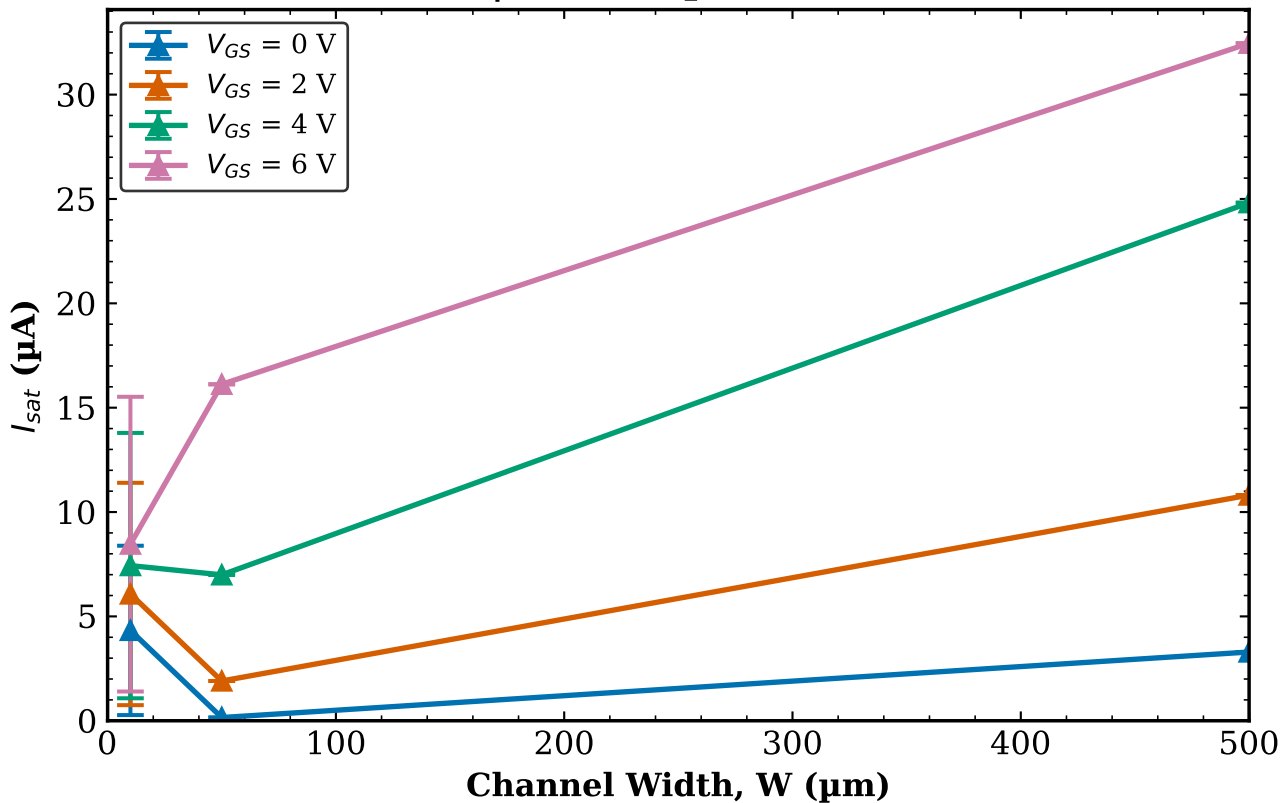
TFT2 Combined (Tr. 1 & 2) I_{sat} vs W | L = 40\text{ }\mu\text{m} (mean \pm std)
